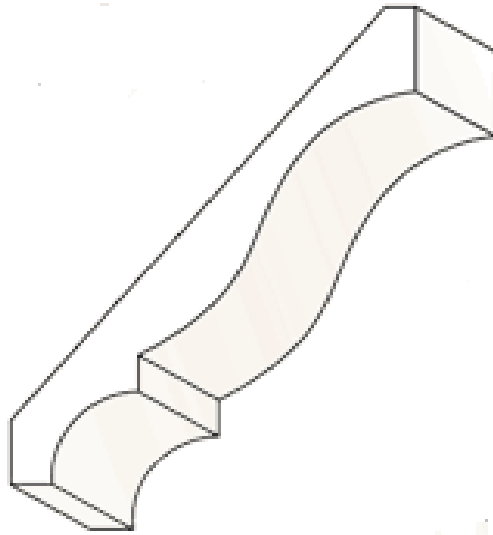
Columbus Wood Products: Crown Moulding C-47 9/16" X 5 5/8"
